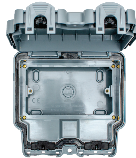
2 GANG ENCLOSURE IP66 173x163x90mm
