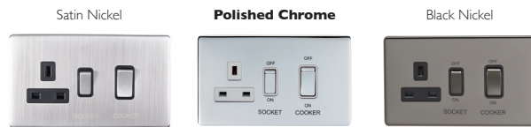
45 AMP DP COOKER SWITCH WITH 13 AMP SOCKET 146x86x6mm
