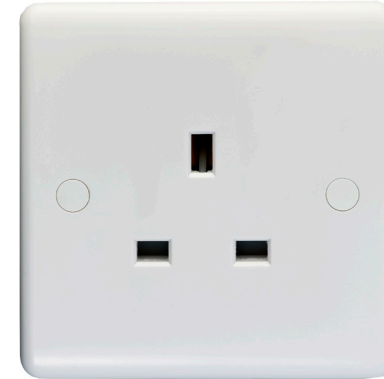
13A 1 GANG UNSWITCHED SOCKET 86x86x7mm
